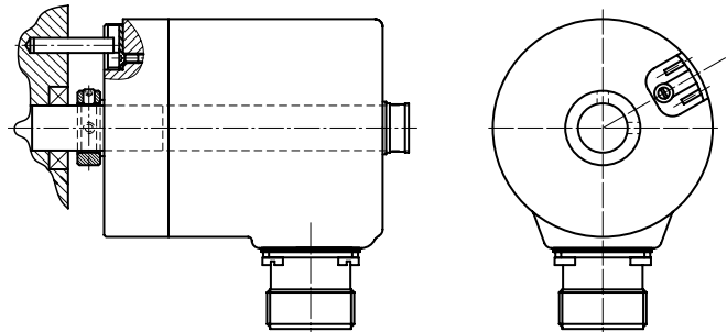
Recessed hollow shaft encoder
