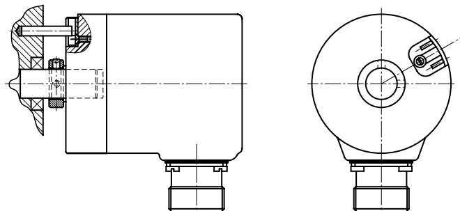
Recessed hollow shaft encoder
